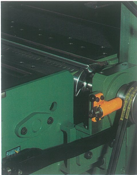
Bottom cutterhead with height adjustment and locking device.
