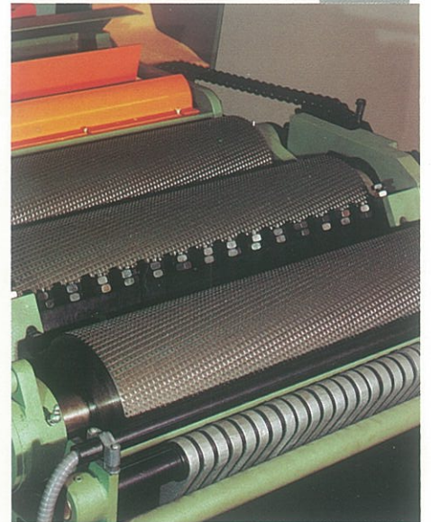
Top infeed rolls of big diameter and sectional holddown.
