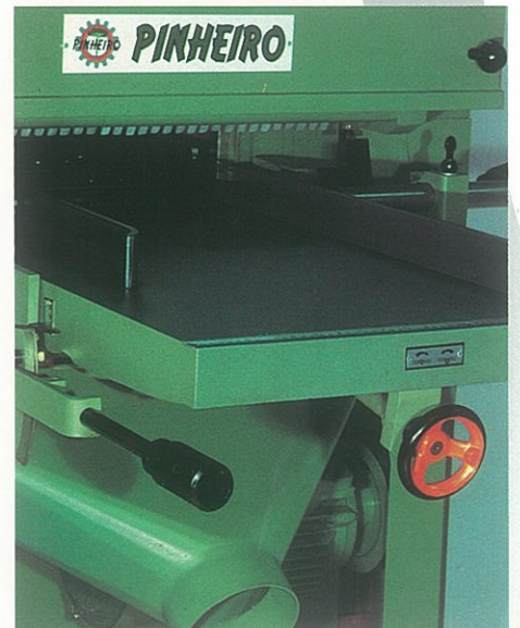
Infeed table and bottom feed rolls height adjustments.
